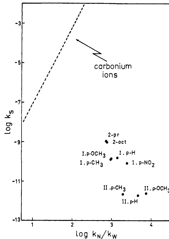
Figure 3. A plot of \log k_s vs. \log k_N/k_W for primary and secondary alkyl chlorides in 80% acetone at 25°.
