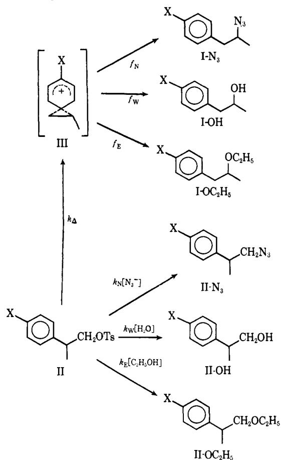
Scheme II. A Kinetic Model for the Solvolysis of 2-Aryl-1-propyl Tosylates in Aqueous Ethanol in the Presence of Sodium Azide
