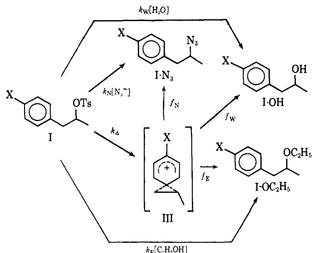
Scheme I. A Kinetic Model for the Solvolysis of 1-Aryl-2-propyl Tosylates in Aqueous Ethanol in the Presence of Sodium Azide
