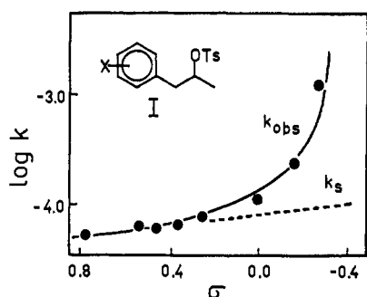
Figure 1. The dissection of the rate constants for the solvolysis of 1-aryl-2-propyl tosylates in 80% ethanol at 75°.
