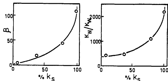
Figure 2. Plots of \beta (rate enhancement) and k_N/k_W (azide incorporation) vs. % k_s for the solvolysis of 1-aryl-2-propyl tosylates in 80% ethanol at 75°.
